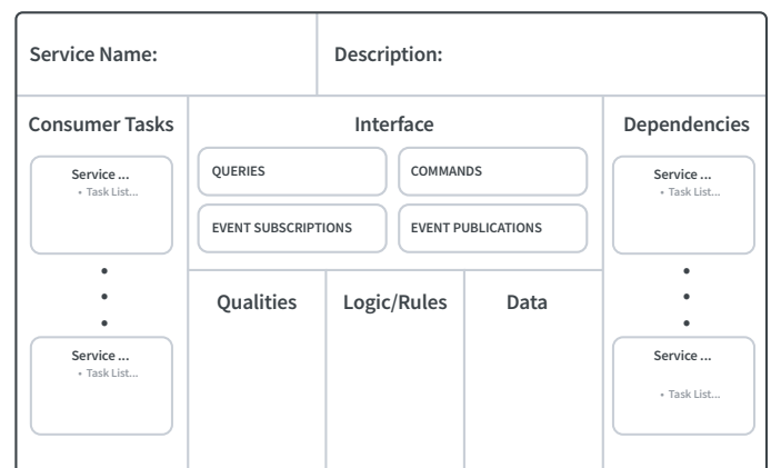
Figure 1 - The Microservice Design Canvas
