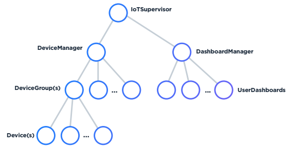
Figure 3: An Actor representation of the IoT architecture.
