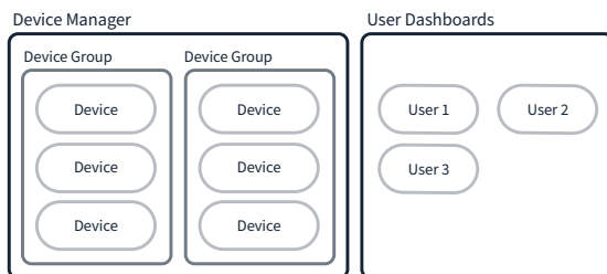
Figure 2: IoT sample application architecture (Source: Akka documentation )
