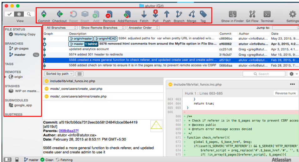
Figure 7.11. Repository details
