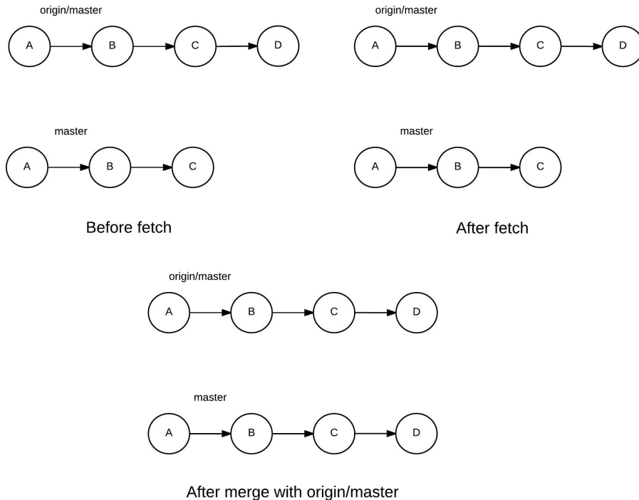
Figure 4.6. Status of the repositories before and after the fetch/merge process
