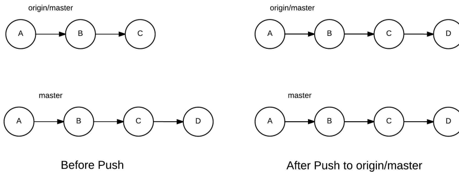
Figure 4.5. The status of a remote after a push operation
