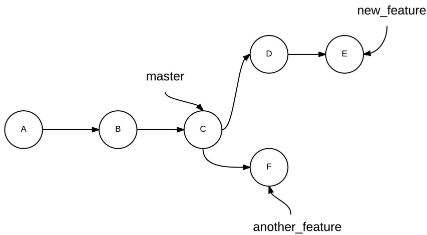
Figure 3.9. Visualizing our branches before the merge
