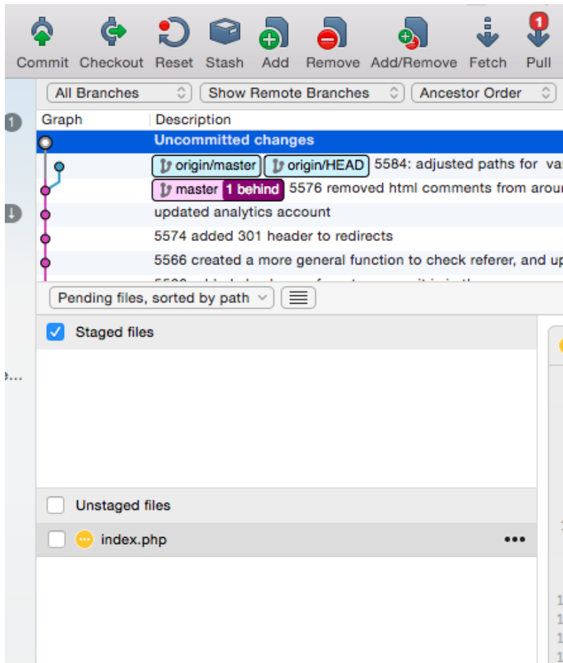
Figure 7.14. Staged and unstaged files following changes to your repository
