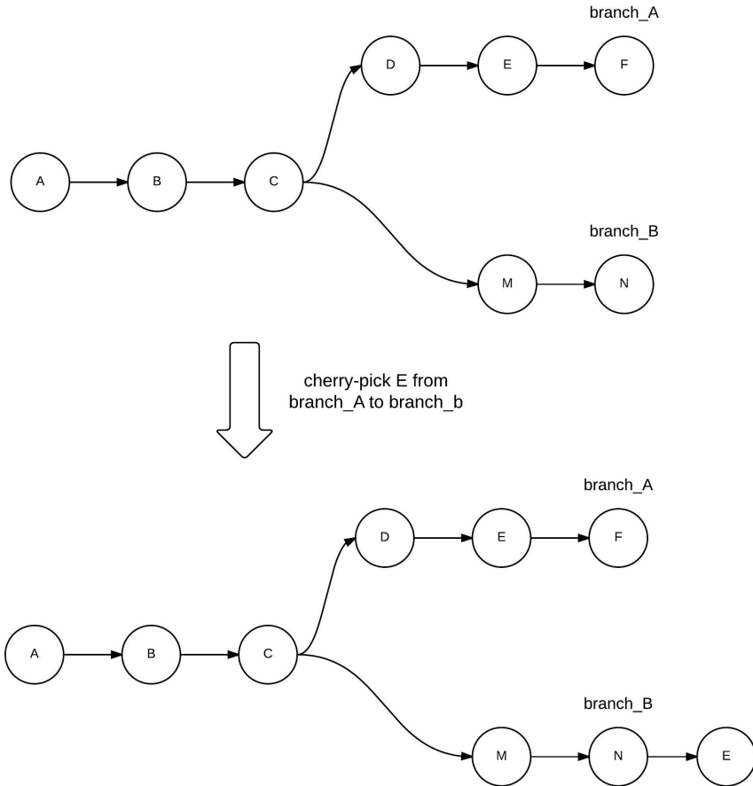
Figure 6.26. Illustration of cherry-pick
