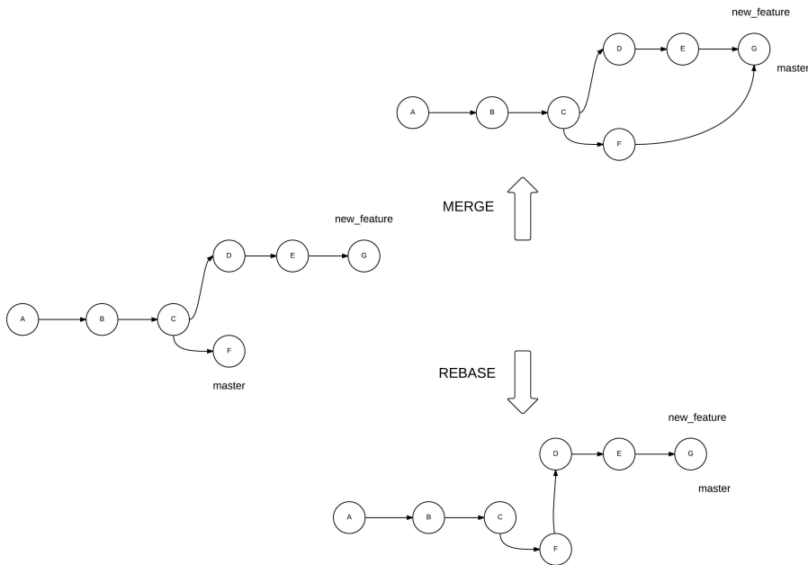
Figure 6.16. Illustrating the difference between merge and rebase
