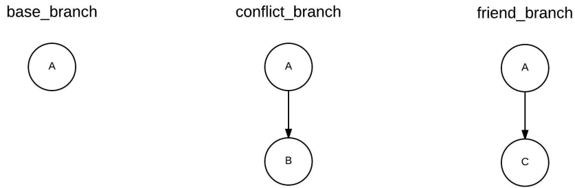
Figure 4.9. A situation where a merge raises a conflict
