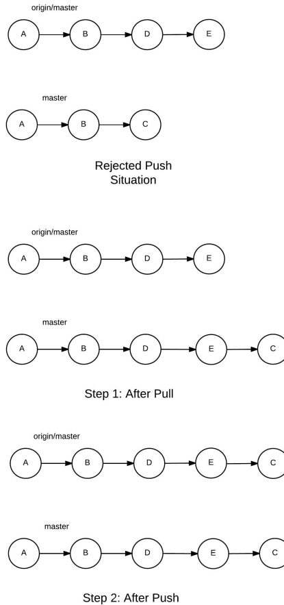
Figure 4.8. Example of a situation where a push is rejected
