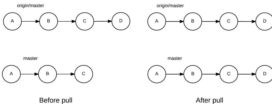
Figure 4.7. Illustration of the status of a local repository before and after a pull
