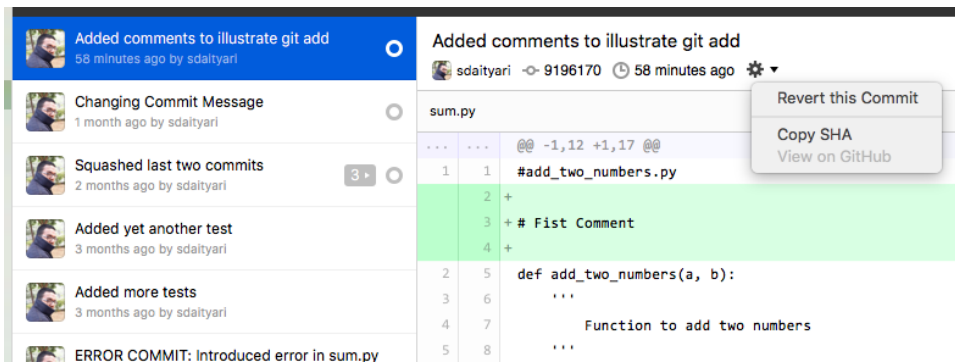
Figure 7.6. Commit options
