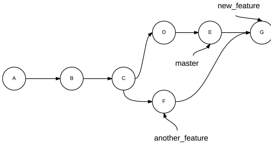
Figure 3.11. The status of the repository after merging another_feature into new_feature
