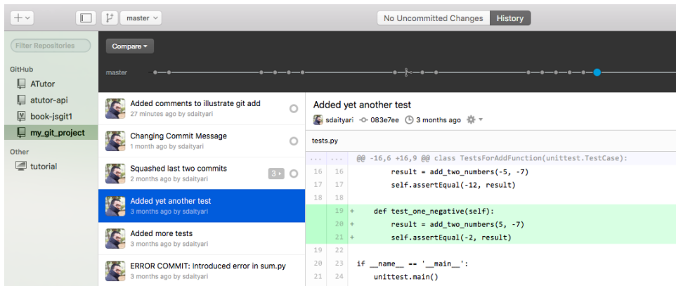
Figure 7.3. Listing the commits in the active branch
