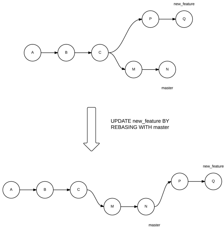
Figure 6.15. Rebase master into new_feature
