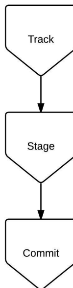
Figure 2.1. Commit workflow
