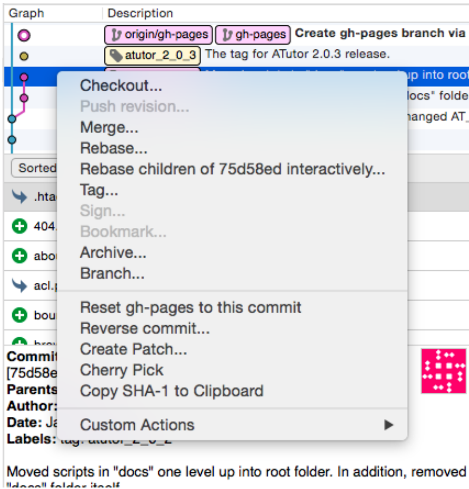
Figure 7.20. Specific operations for a commit
