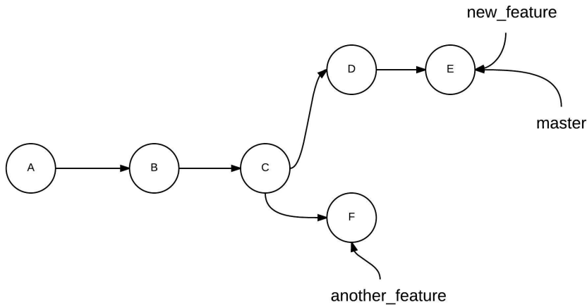
Figure 3.10. The status of the repository after merging new_feature into master
