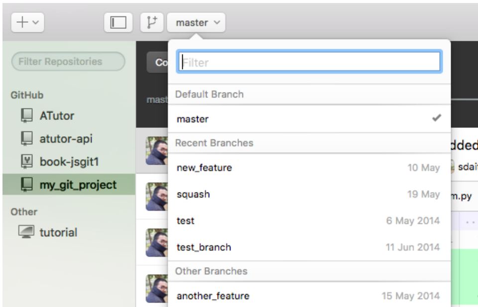
Figure 7.5. Changing the active branch
