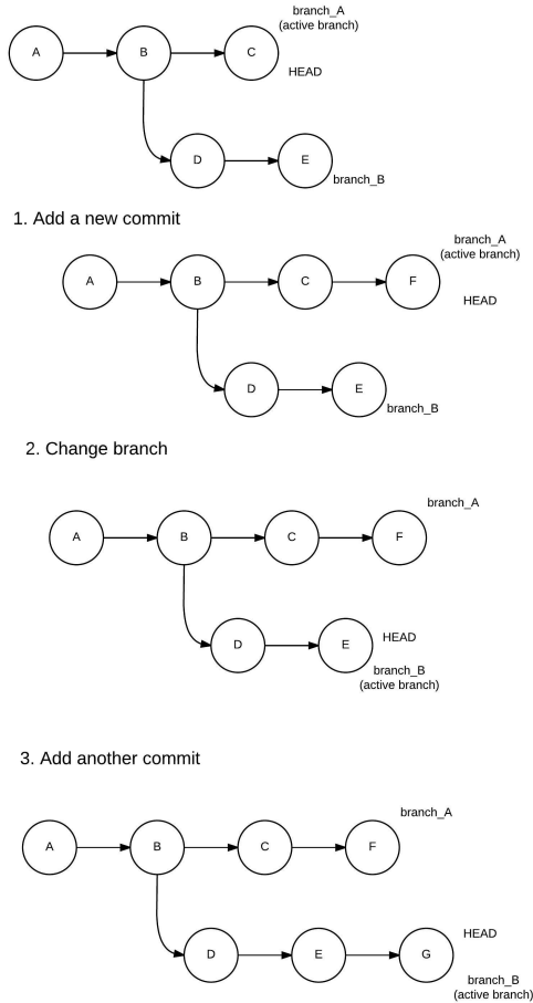
Figure 3.7. Branches and HEAD
